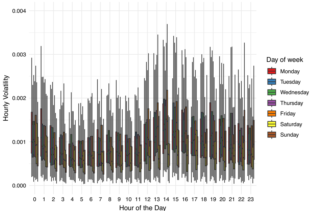
Fig. 2. Distribution of hourly volatility in bitcoin log returns by day of the week.
