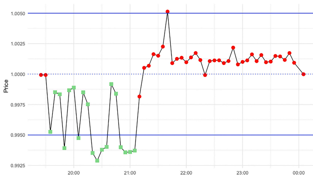
Fig. 3. Tether price with alternative depeg detection.
