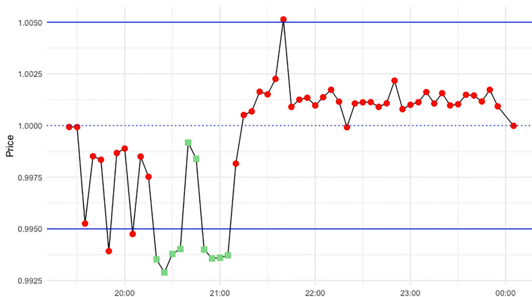
Fig. 1. Tether price with depeg detection.
